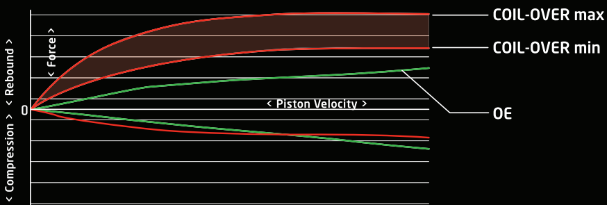
COIL-OVER Damping and Force Comparison
