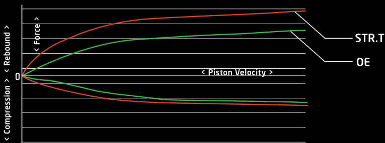
STR.T Damping Force Comparison
