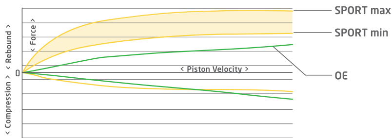
SPORT Damping Force Comparison
